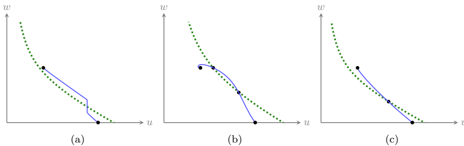
Figure 12: Schematics of other possible solution trajectories.
