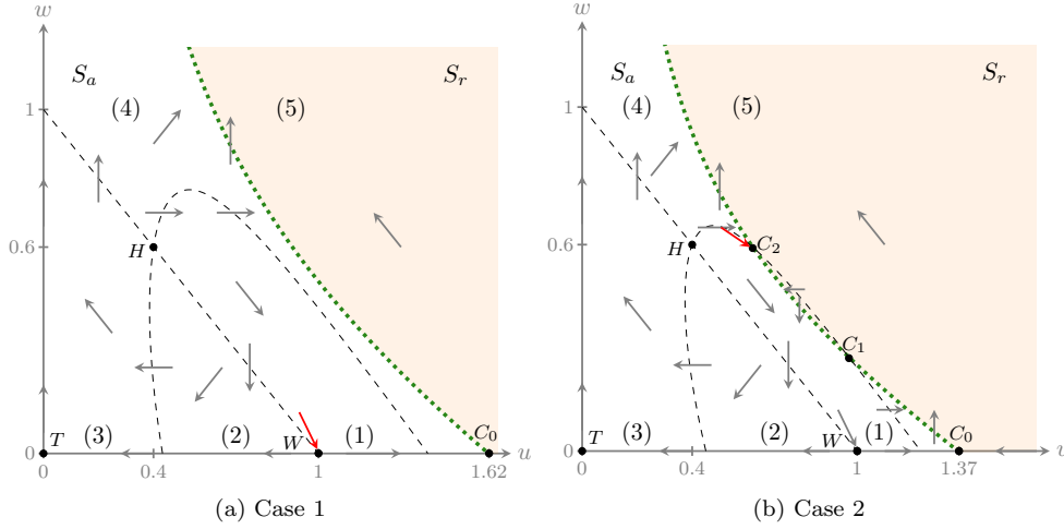
Figure 7: Solution direction of the desingularised system (15) within the different regions of the phase planes, separated by the nullclines. Once again, the green dotted line and the black dashed lines correspond to the nullclines of (15) and the black circles to the equilibria, with the green dotted line also coinciding with the wall of singularities (5). The red arrows indicate the directions of the stable eigenvector of the linearised system at the equilibria of interest. The equilibria are labelled according to Table 1.
