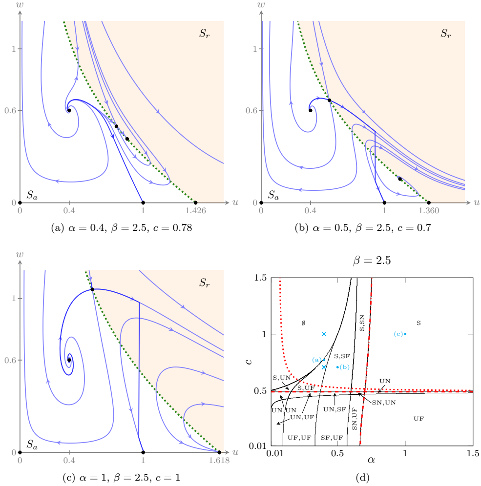
Figure 11: Illustrations of the different solution behaviours observed within the same region of parameter space as Case 2 and similar solution behaviours observed in other regions of parameter space. The last panel indicates the locations in parameter space of the parameters used to construct the three phase planes. The first panel depicts a smooth connection in the presence of canard points (in the same region as Case 2), the second and third panels depict two parameter regimes (in different regions to Case 2) where heteroclinic orbits containing a jump can be constructed.
