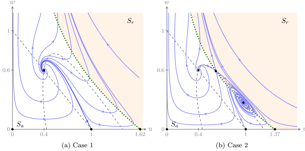
Figure 6: Phase planes of (15) under the two parameter regimes. The green dotted line and the black dashed lines correspond to the nullclines of the system and the black circles to the equilibria. Note that both axes are also nullclines. Moreover, the green dotted line coincides with F .
