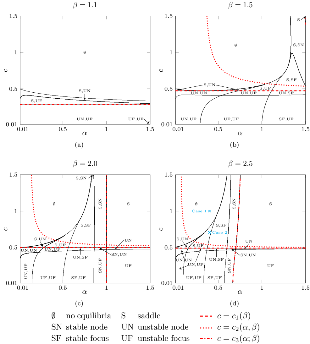
Figure 5: Illustration of the number and stability of the equilibria (u_{C_k}, w_{C_k}) of (15), with 0 < u_{C_k} < u_{C_0} , for different parameter values. The points corresponding to the locations of the Case 1 and Case 2 parameter regimes are marked \times . In both cases (u_H, w_H) is an unstable focus since c > c_2(\alpha, \beta) . Note that for the parameter ranges shown here, we do not observe any saddle equilibria for c < c_1(\beta) .
