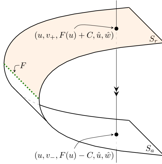
Figure 4: A schematic of the critical manifold S and the flow through the layer problem.
