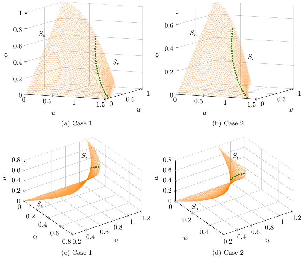
Figure 3: The critical manifold S defined in (13) projected into (u, w, \hat{w}) -space, for Case 1 and Case 2. The green dotted line corresponds to the fold curve F .
