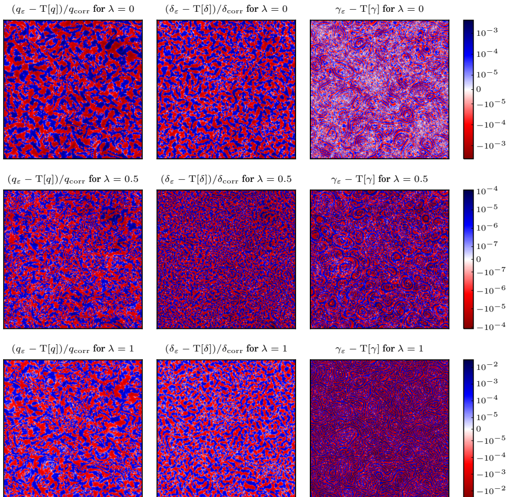
FIGURE 5. Late time relative differences (at \varepsilon t = 1 ) of the difference between shallow water fields and corresponding transformed balance model fields. All other parameters and normalizing values are the same as in Figure 4. Note that the color scales are the same as for the corresponding rows in Figure 4 so that the growth in color saturation gives an impression of the growth in the error as time progresses.
