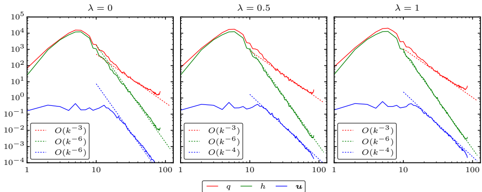
FIGURE 9. Power density spectra for the balance model q , h , and \mathbf{u} for \varepsilon = 2^{-3} , and for different values of \lambda at time \varepsilon t = 1 .
