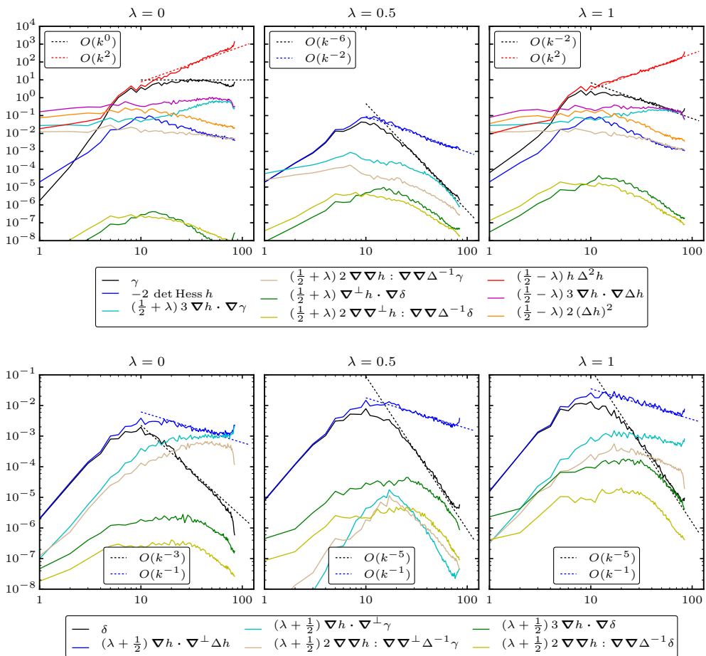
FIGURE 10. Power density spectra for each of the terms on the right hand side of the \gamma -equation (3.27b), upper panel, and of the \delta -equation (3.27a), lower panel, corresponding to the case shown in Figure 9.
